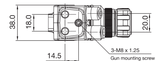
Mounting dimensions (mm)
